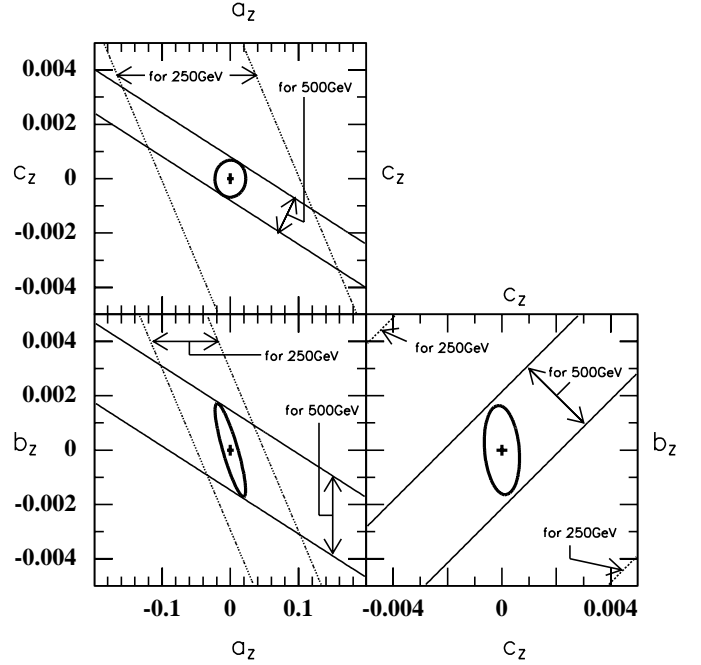
Fig. 5. The projections of the \chi^2 = 1 contours onto the (a_Z, b_Z) , (b_Z, c_Z) and (c_Z, a_Z) planes for \sqrt{s} = 250 GeV and 500 GeV. The central values of a_Z , b_Z and c_Z are assumed to coincide with their SM values, a_Z = b_Z = c_Z = 0 . The errors are estimated under the condition \epsilon_\tau = 0.4 , \epsilon_b = 0.2 and |P| = 0.9 . Dashed (thin solid) lines represent the one- \sigma contours obtained at \sqrt{s} = 250 (500) GeV. Thick solid curves represent the combined one- \sigma contours
