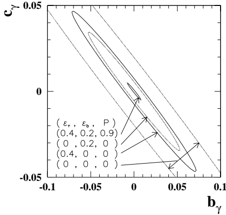
Fig. 2. Contours of \chi^2 = 1 in the (b_\gamma, c_\gamma) plane for \sqrt{s} = 250 GeV. The other degrees of general couplings are integrated out. The central values of b_\gamma and c_\gamma are assumed to coincide with their SM values, b_\gamma = c_\gamma = 0 . The errors are estimated by means of the optimal-observable method under the following four conditions: a \epsilon_\tau = \epsilon_b = P = 0 ; b \epsilon_\tau = 0.4 and \epsilon_b = P = 0 ; c \epsilon_b = 0.2 and \epsilon_\tau = P = 0 ; or d \epsilon_\tau = 0.4 , \epsilon_b = 0.2 and |P| = 0.9
