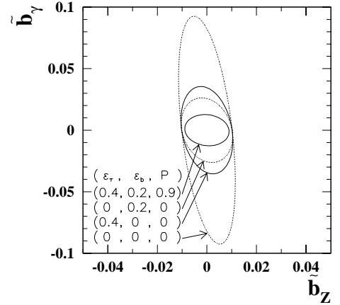
Fig. 4. Contours of \chi^2 = 1 in the (\tilde{b}_Z, \tilde{b}_\gamma) plane for \sqrt{s} = 250 GeV. The other degrees of general couplings are integrated out. The central values of \tilde{b}_Z and \tilde{b}_\gamma are assumed to coincide with their SM values, \tilde{b}_Z = \tilde{b}_\gamma = 0
