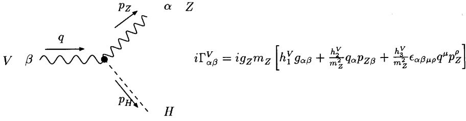
Fig. 1. General HZV coupling. The arrows indicate the direction of the four-momentum flow
