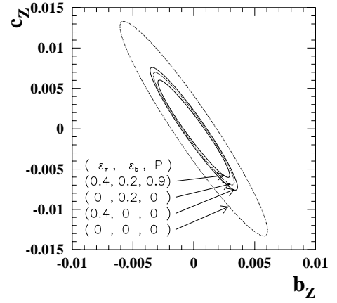
Fig. 3. Contours of \chi^2 = 1 in the (b_Z, c_Z) plane for \sqrt{s} = 250 GeV. a_Z = 0 and the other degrees of general couplings are integrated out. The central values of b_Z and c_Z are assumed to coincide with their SM values, b_Z = c_Z = 0
